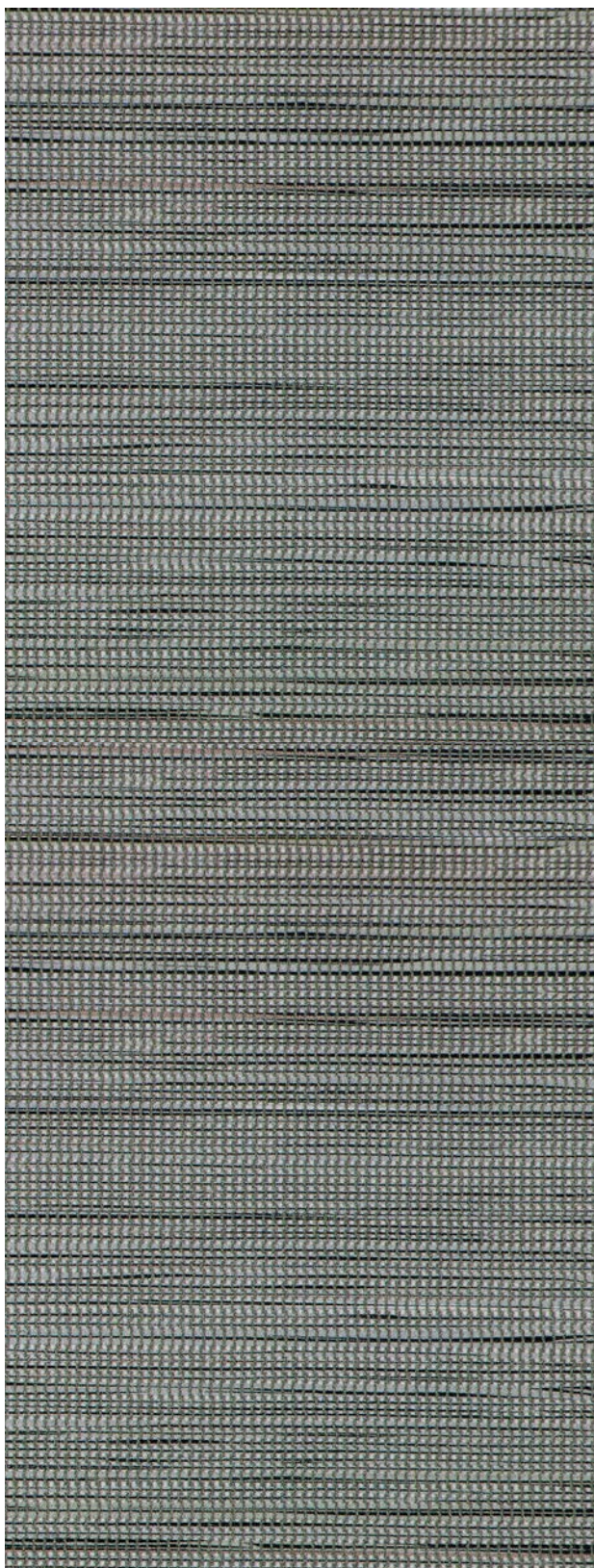
Granite
