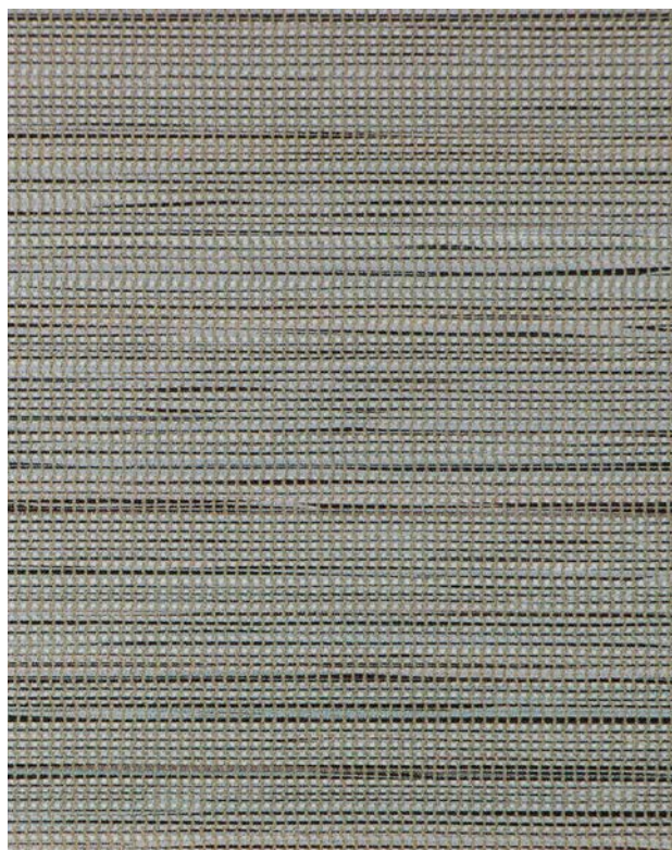
Quartz
